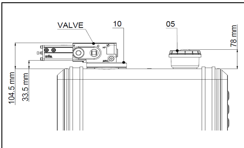
Valve mounted on top of tank
