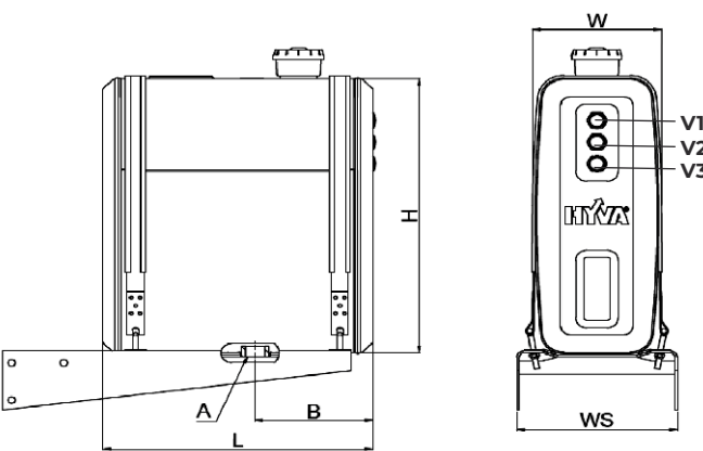
14016580K + 14016581K (TANK + SUPPORT ON CRADLE)
