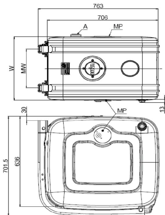
Double support tank
