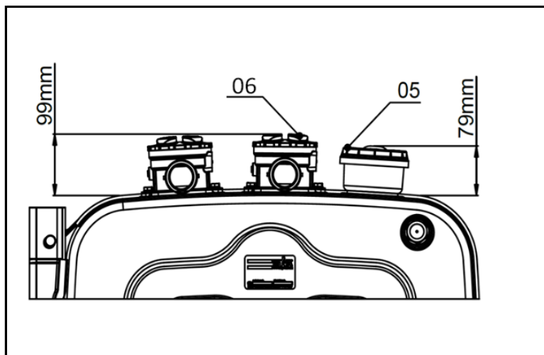
Valve mounted on chassis or cylinder (SAE)
