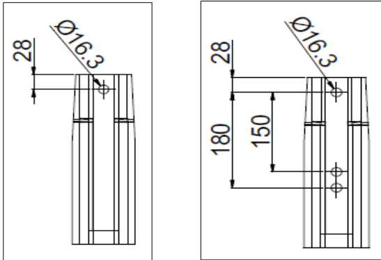
Detail support with one hole and support with three holes
