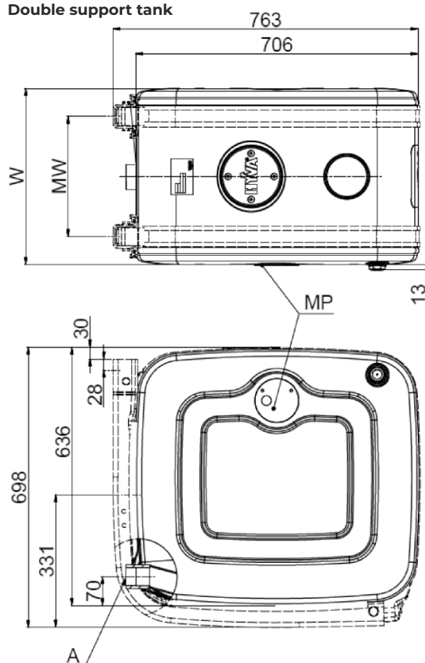
Double support tank
