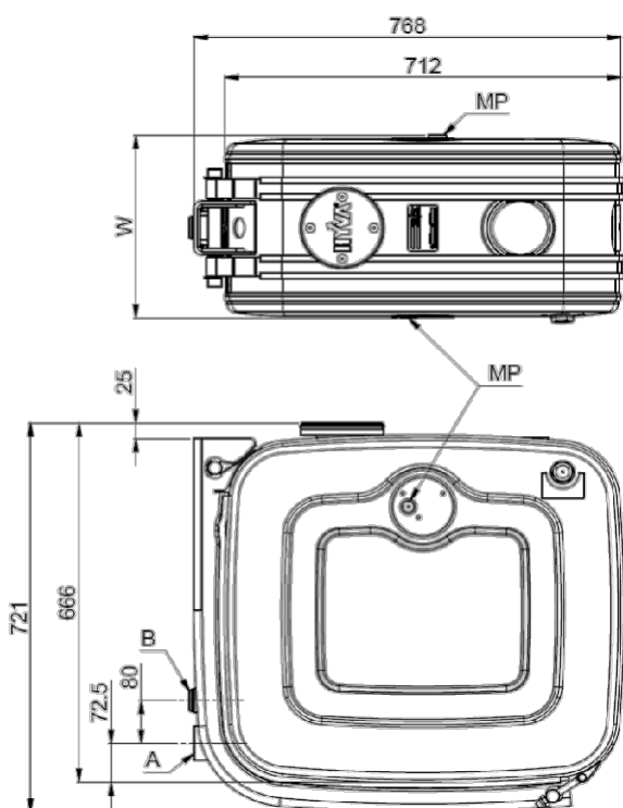
Single support tank
