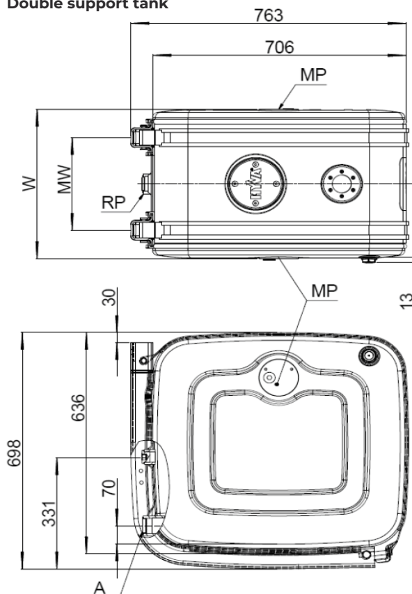
Double support tank
